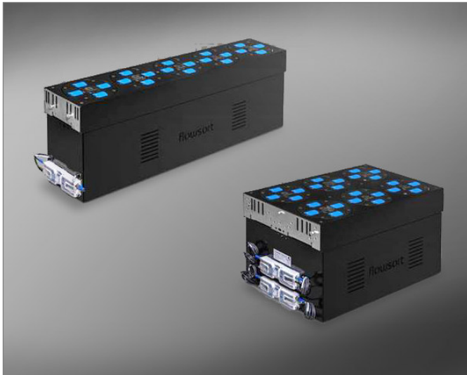
Modular high-speed diverter from Flowsort on a 24-volt basis for sorting up to 8000 units with a weight of 50 g to 35 kg (Picture source: Flowsort B.V.)
